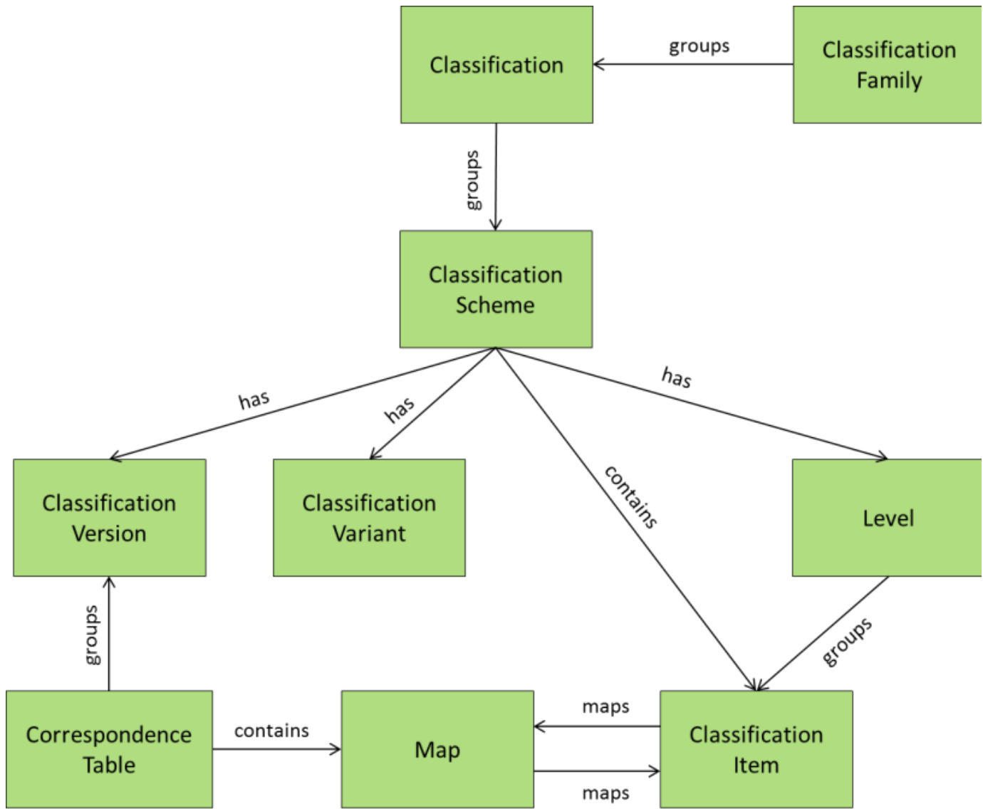
Figure 15. Over view of Classification
