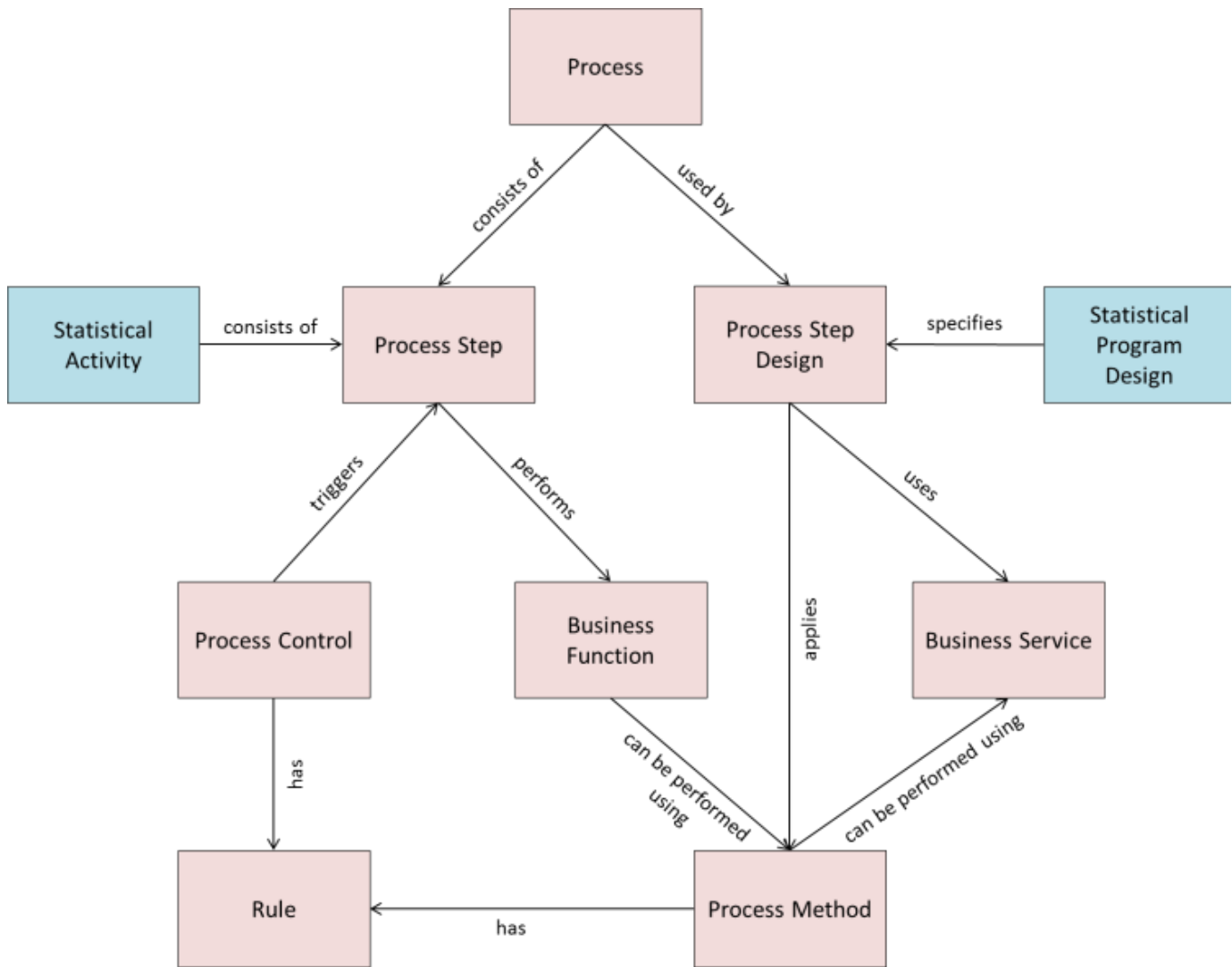
Figure 7. Simplified view of Production Group objects
