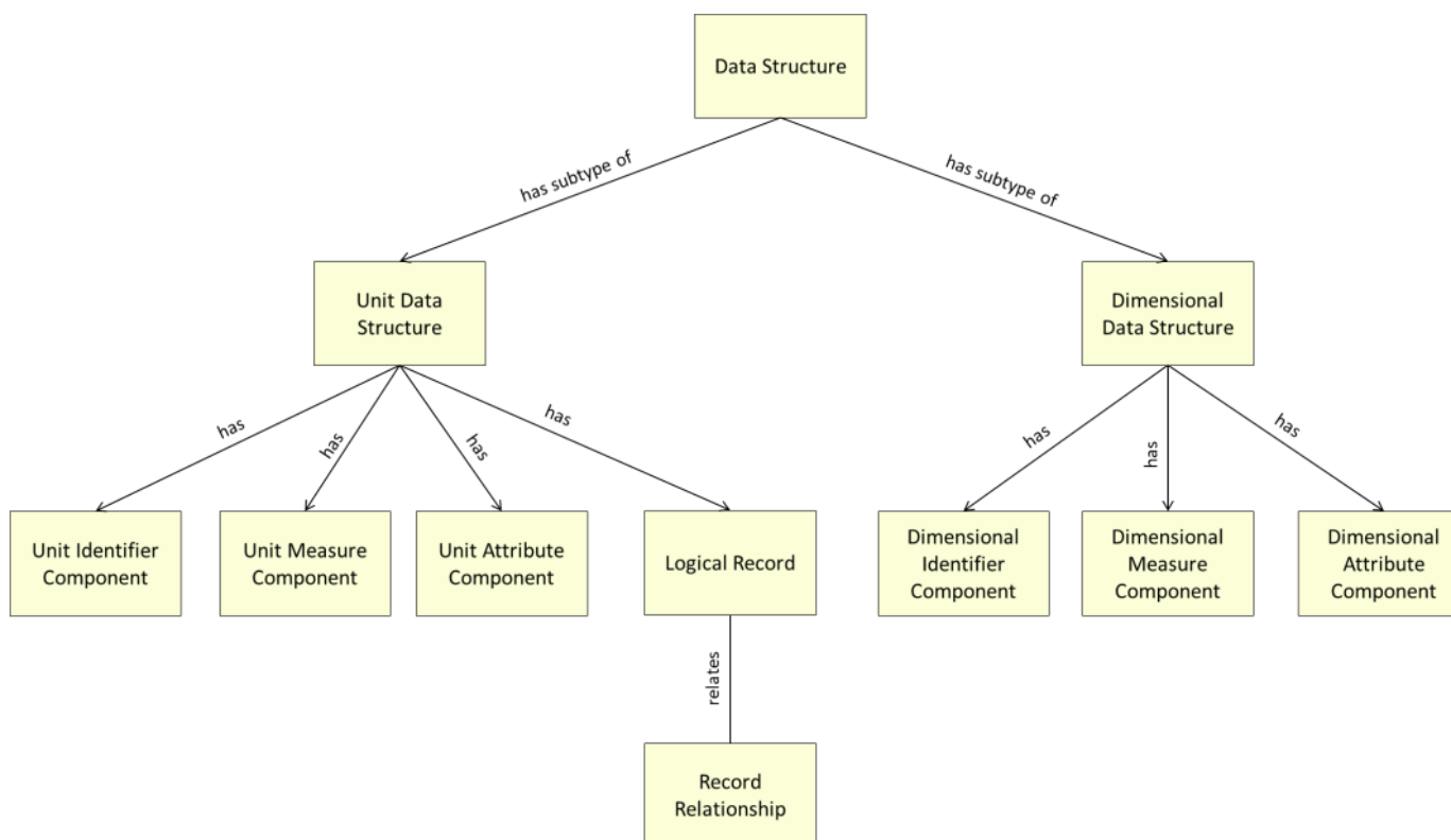
Figure 19. Dimensional and Unit Data Structures
