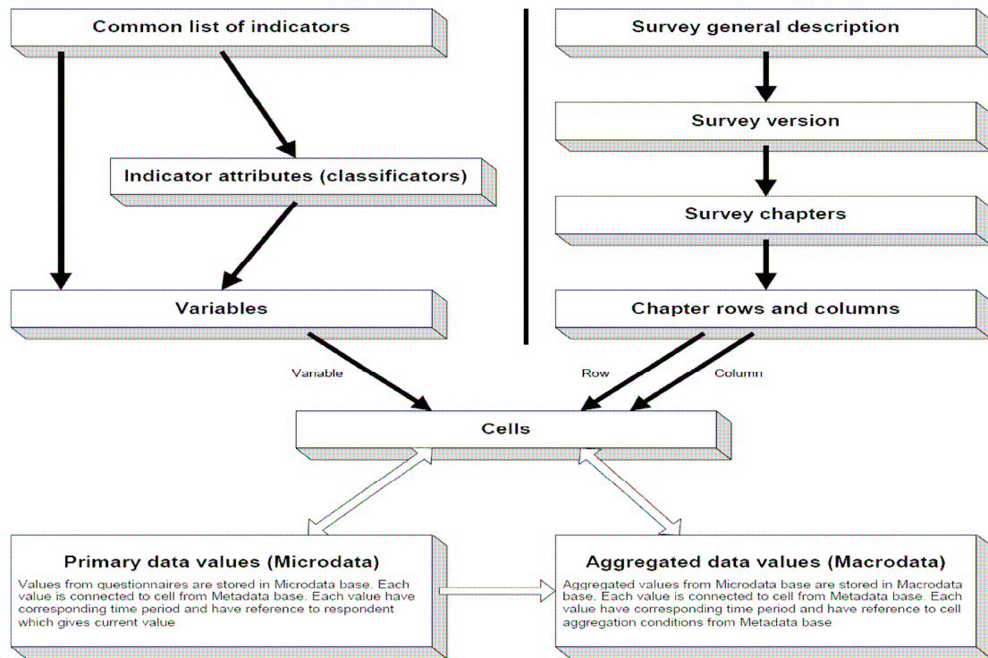
Figure 2 – Meta data base link with Micro and Macro data bases
